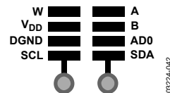
Figure 41. Recommended AD5273 PCB Layout
