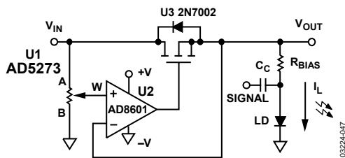
Figure 47. Programmable Booster Voltage Source
