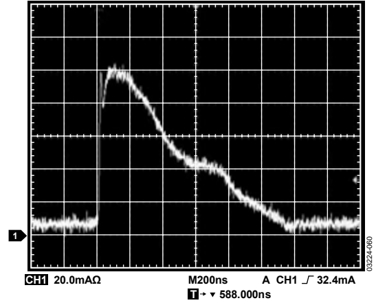
Figure 28. OTP Program Energy Plot
